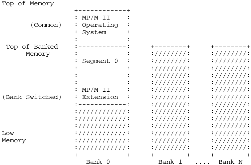
Figure 1-1. MP/M II Memory Organization
